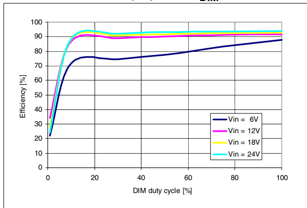
Figure 5. Efficiency vs DIM duty cycle @ f_{DIM} = 1\text{ kHz}
