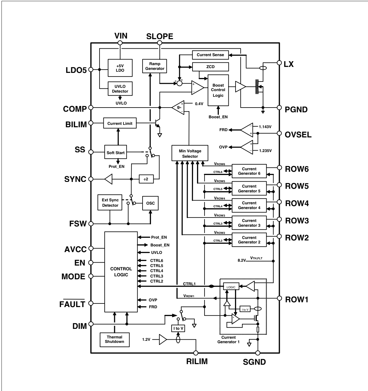
Figure 42. Simplified block diagram
