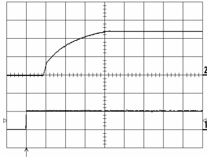
Start-up enabled by connecting V_1 at: T_{P1} = +25^\circ\text{C} , V_1 = 53\text{ V} , I_O = 4.2\text{ A} resistive load. Top trace: output voltage (5 V/div.). Bottom trace: input voltage (50 V/div.). Time scale: (5 ms/div.).
