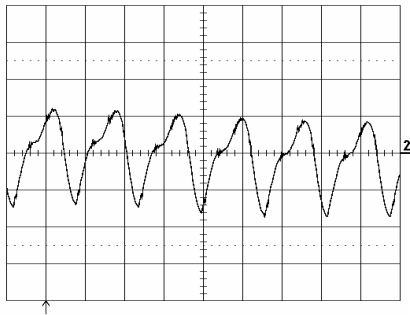
Output voltage ripple at: T_{P1} = +25^\circ\text{C} , V_1 = 53\text{ V} , I_O = 4.2\text{ A} resistive load. Trace: output voltage (20 mV/div.). Time scale: (2 \mu\text{s} /div.).
