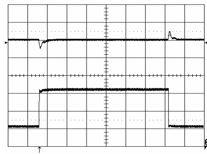
Output voltage response to load current step-change (1.05 - 3.15 - 1.05 A) at: T_{P1} = +25^\circ\text{C} , V_1 = 53\text{ V} . Top trace: output voltage (1 V/div.). Bottom trace: load current (1 A/div.). Time scale: (0.1 ms/div.).
