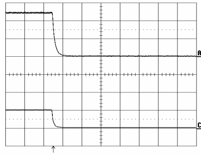
Shut-down enabled by disconnecting V_1 at: T_{P1} = +25^\circ\text{C} , V_1 = 53\text{ V} , I_O = 4.2\text{ A} resistive load. Top trace: output voltage (5 V/div.). Bottom trace: input voltage (50 V/div.). Time scale: (0.2 ms/div.).
