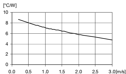
Thermal resistance vs. airspeed measured at the converter. Tested in wind tunnel with airflow and test conditions as per the Thermal consideration section. V_i = 53\text{ V} .
