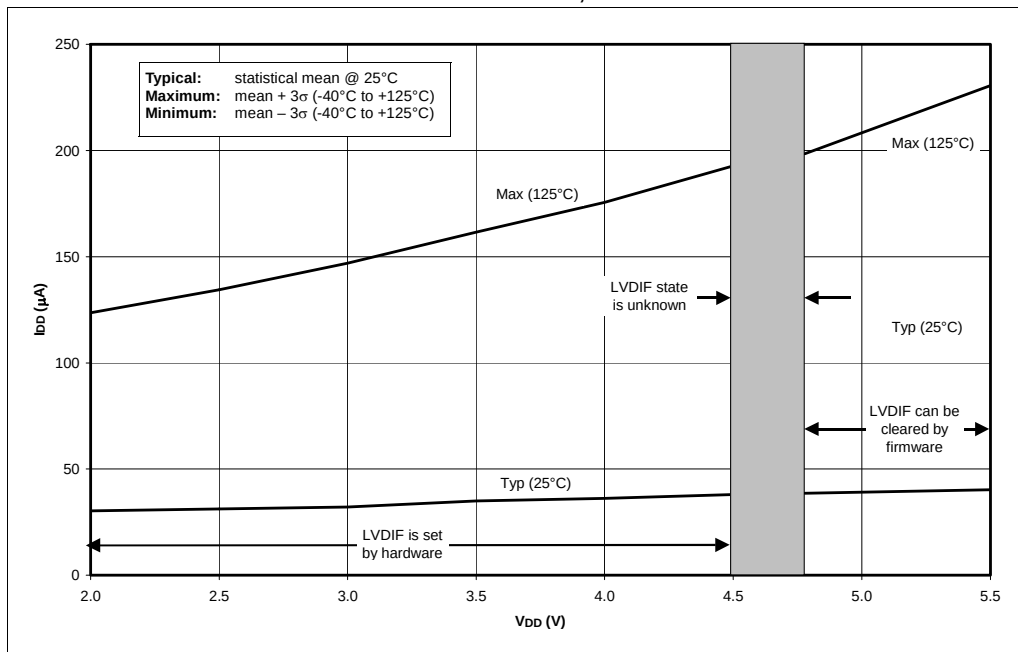
FIGURE 28-20: \Delta I_{LVD} vs. VDD OVER TEMPERATURE, V_{LVD} = 4.5\text{--}4.78\text{V}
