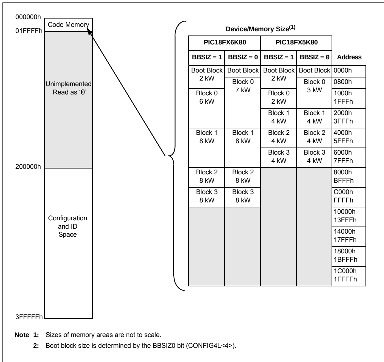
FIGURE 28-6: CODE-PROTECTED PROGRAM MEMORY FOR THE PIC18F66K80 FAMILY
