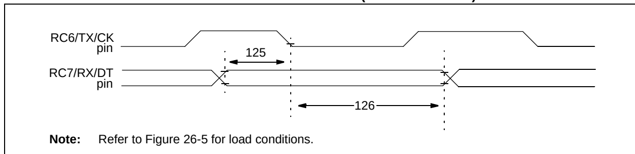
FIGURE 26-22: EUSART SYNCHRONOUS RECEIVE (MASTER/SLAVE) TIMING
