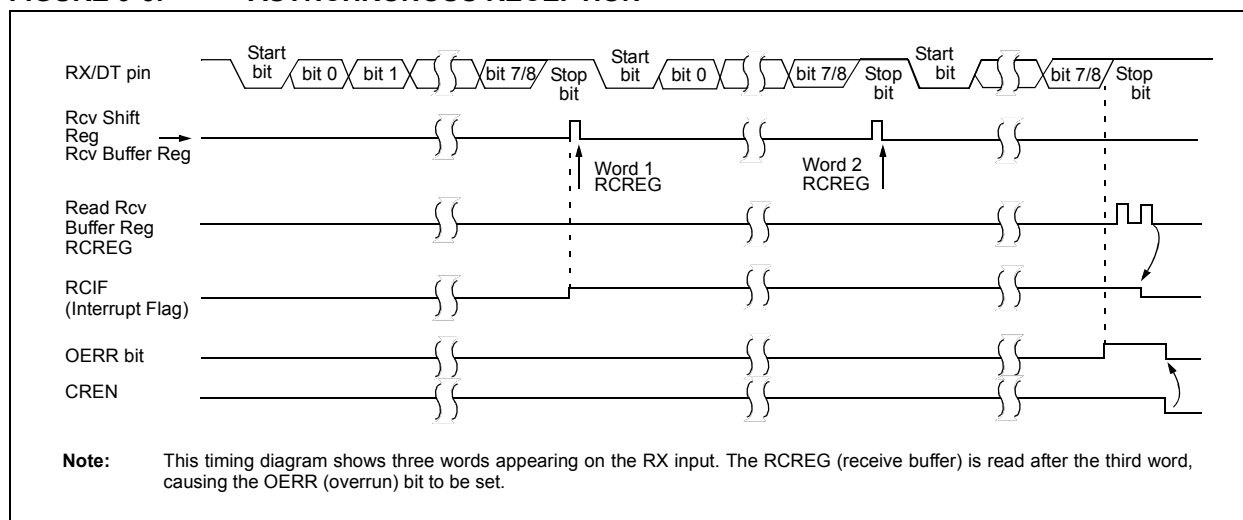
FIGURE 9-5: ASYNCHRONOUS RECEPTION
