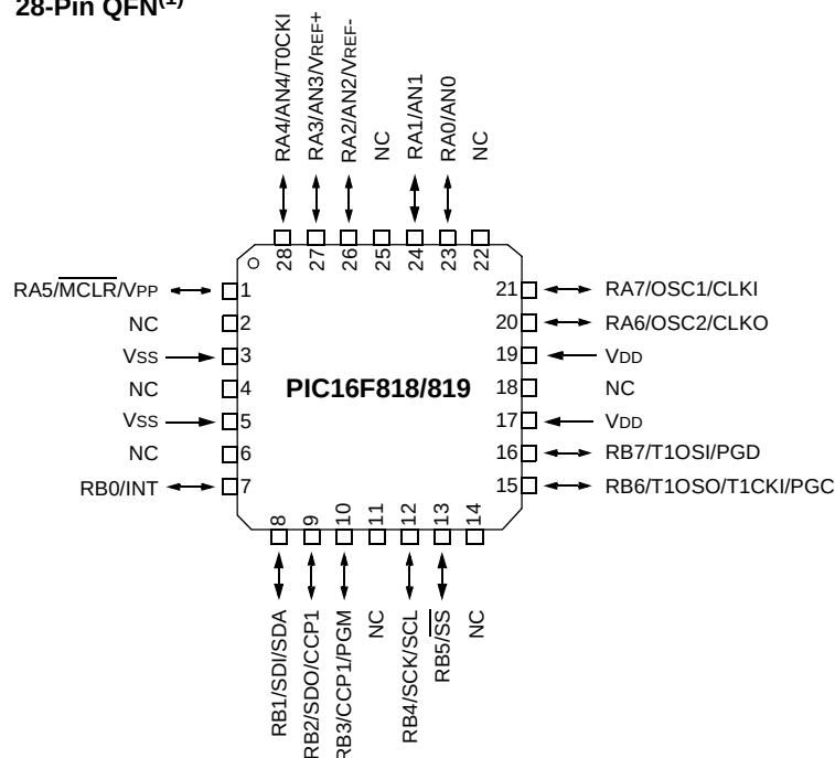
28-Pin QFN (1)
