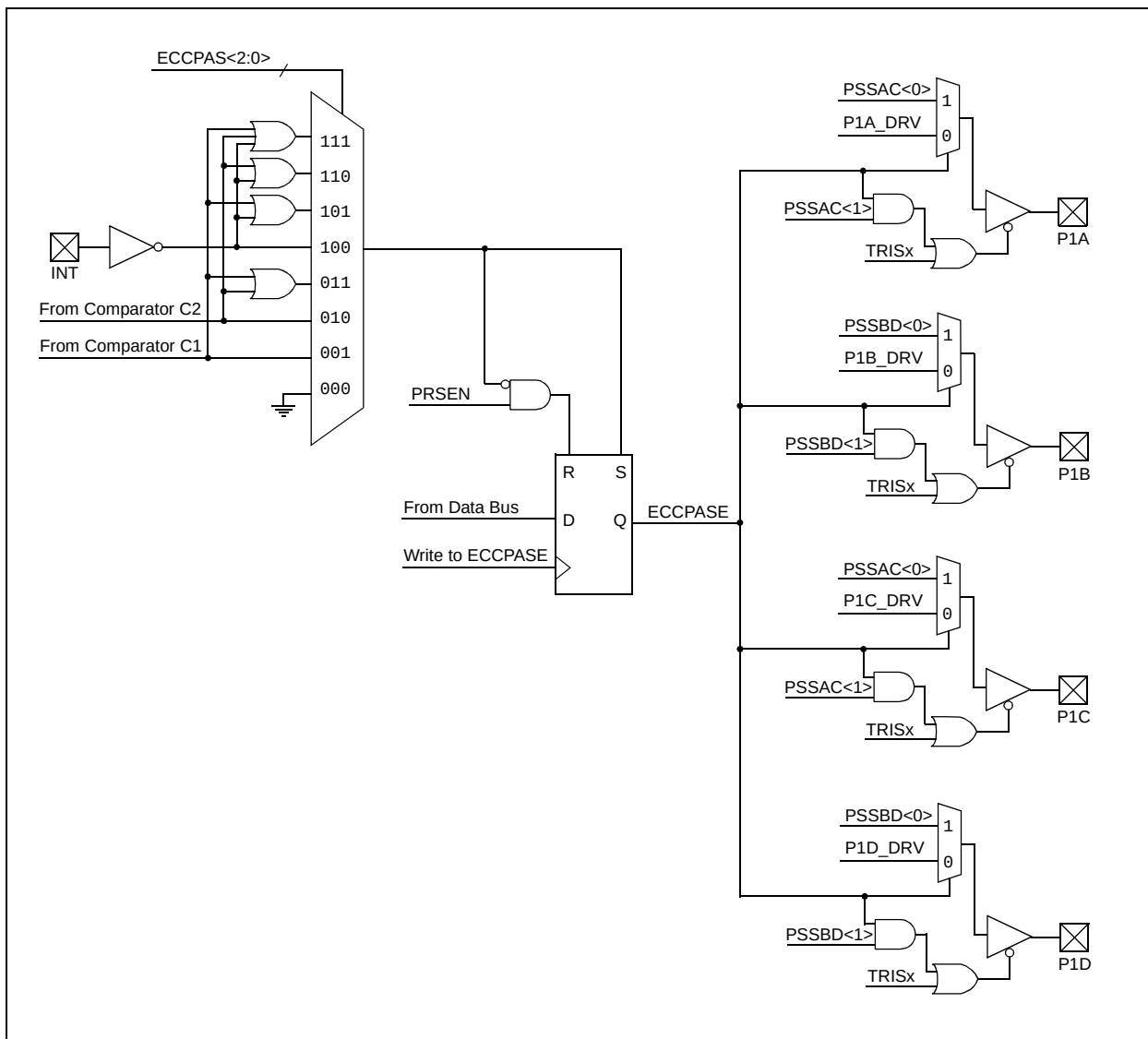
FIGURE 11-14: AUTO-SHUTDOWN BLOCK DIAGRAM
