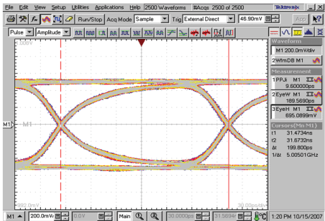
Tx Eye Diagram, 5.0 Gbps
