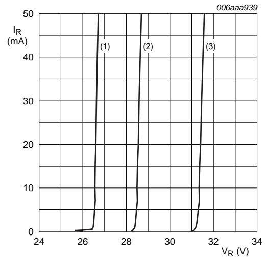
(1) T_{\text{amb}} = -55 \text{ }^\circ\text{C} (2) T_{\text{amb}} = 25 \text{ }^\circ\text{C} (3) T_{\text{amb}} = 150 \text{ }^\circ\text{C}
