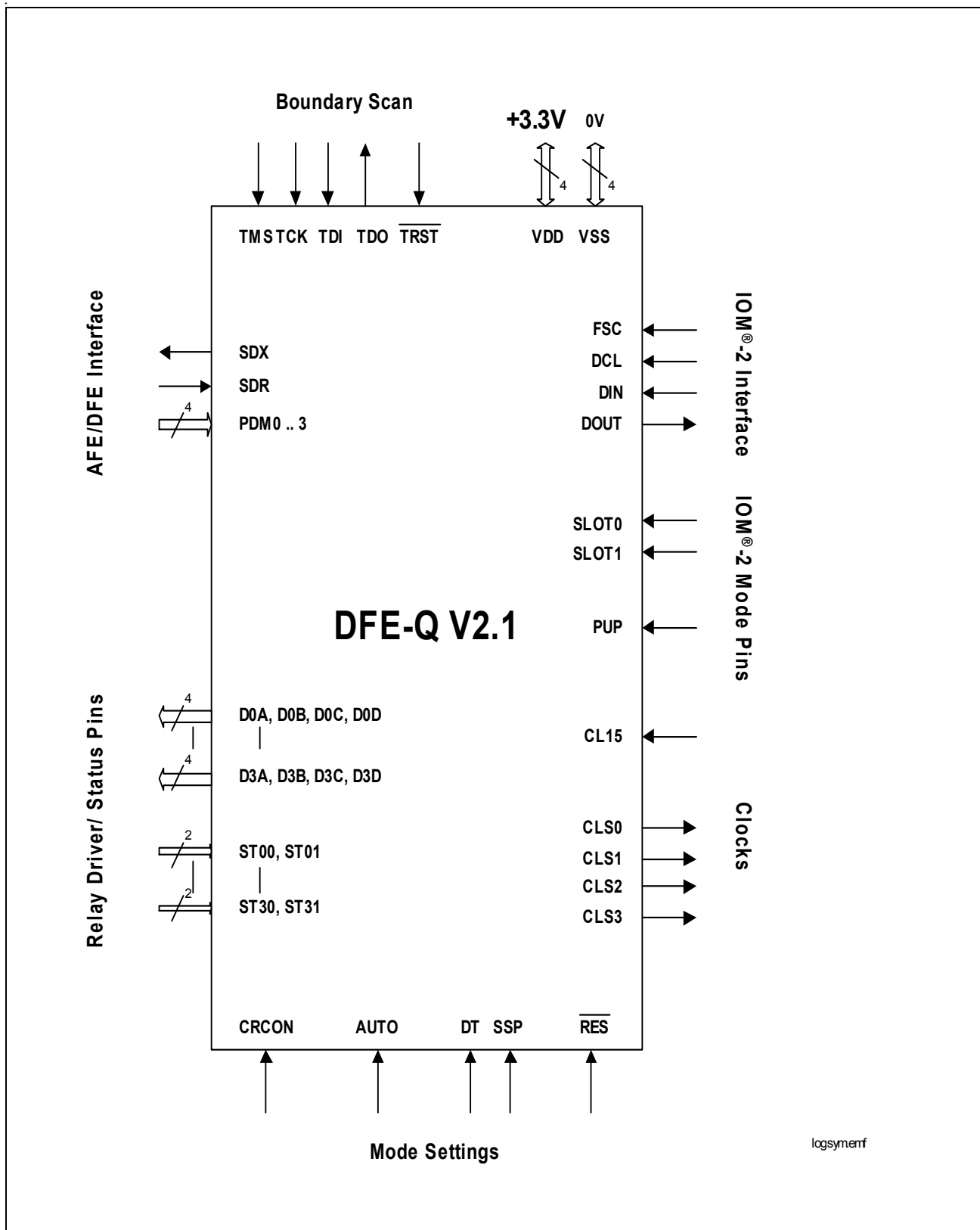
Figure 2 Logic Symbol
