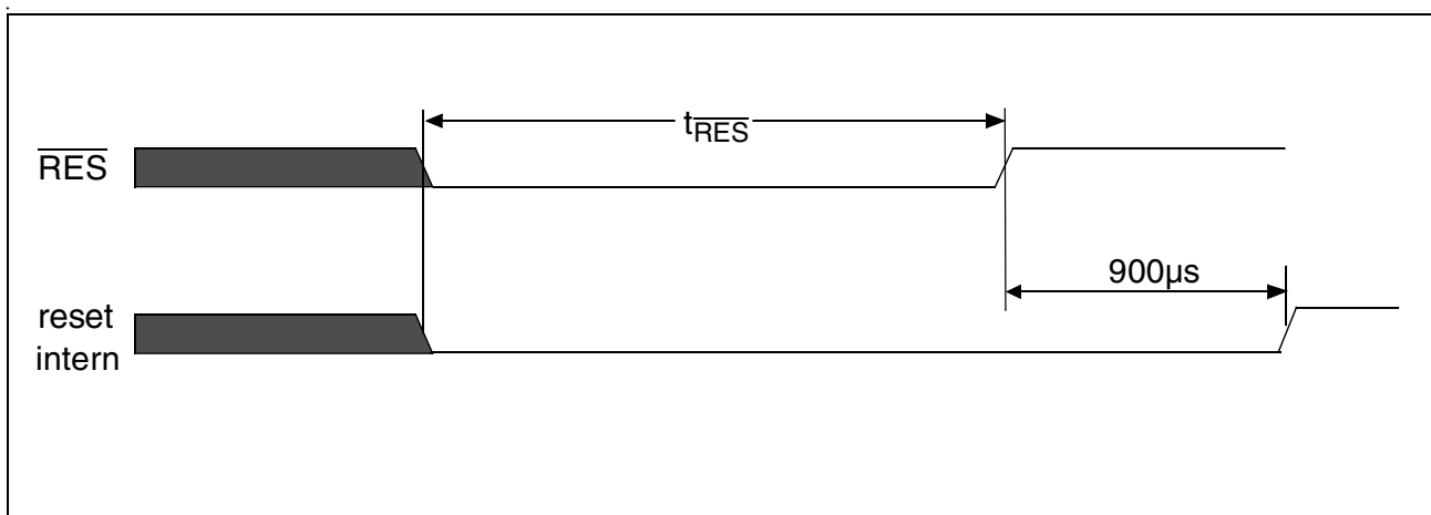
Figure 44 Reset Timing
