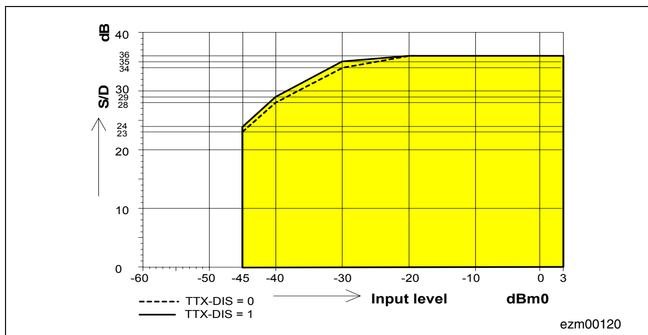
Figure 80 Total Distortion Transmit (L x = 0 dBr)
