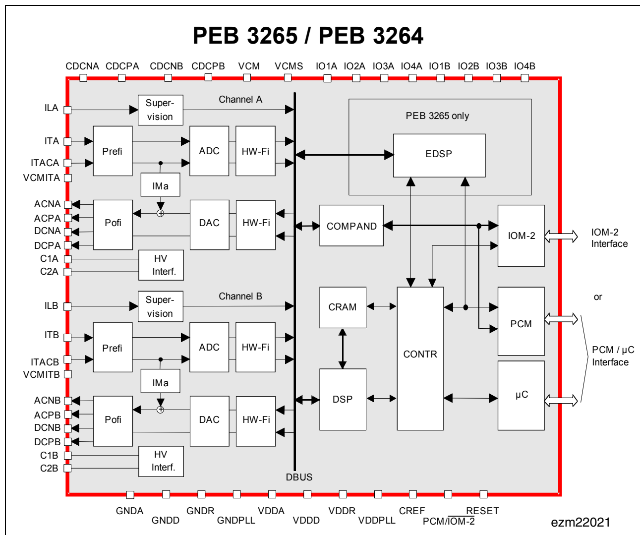
Figure 9 Block Diagram: SLICOFI-2/-2S (PEB 3265, PEB 3264)
