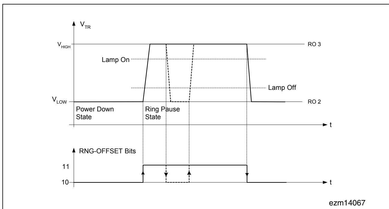
Figure 34 Timing Diagram
