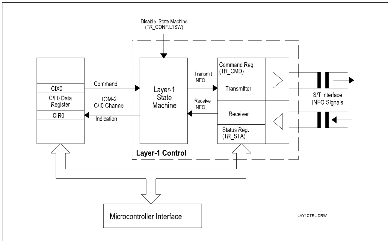
Figure 37 Layer-1 Control
