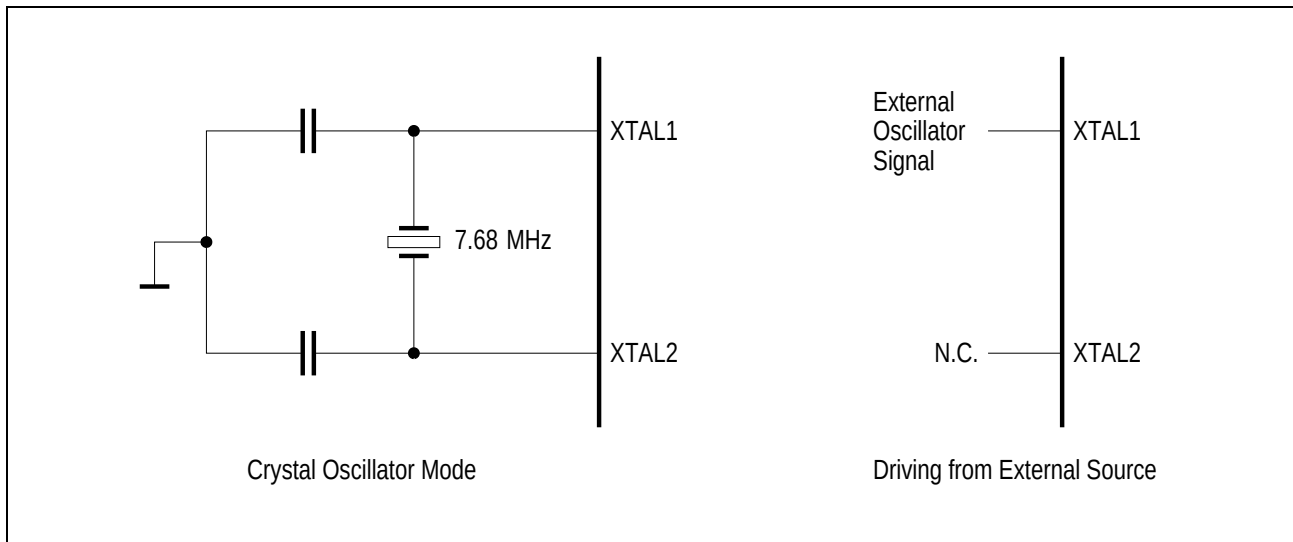
Figure 82 Oscillator Circuits
