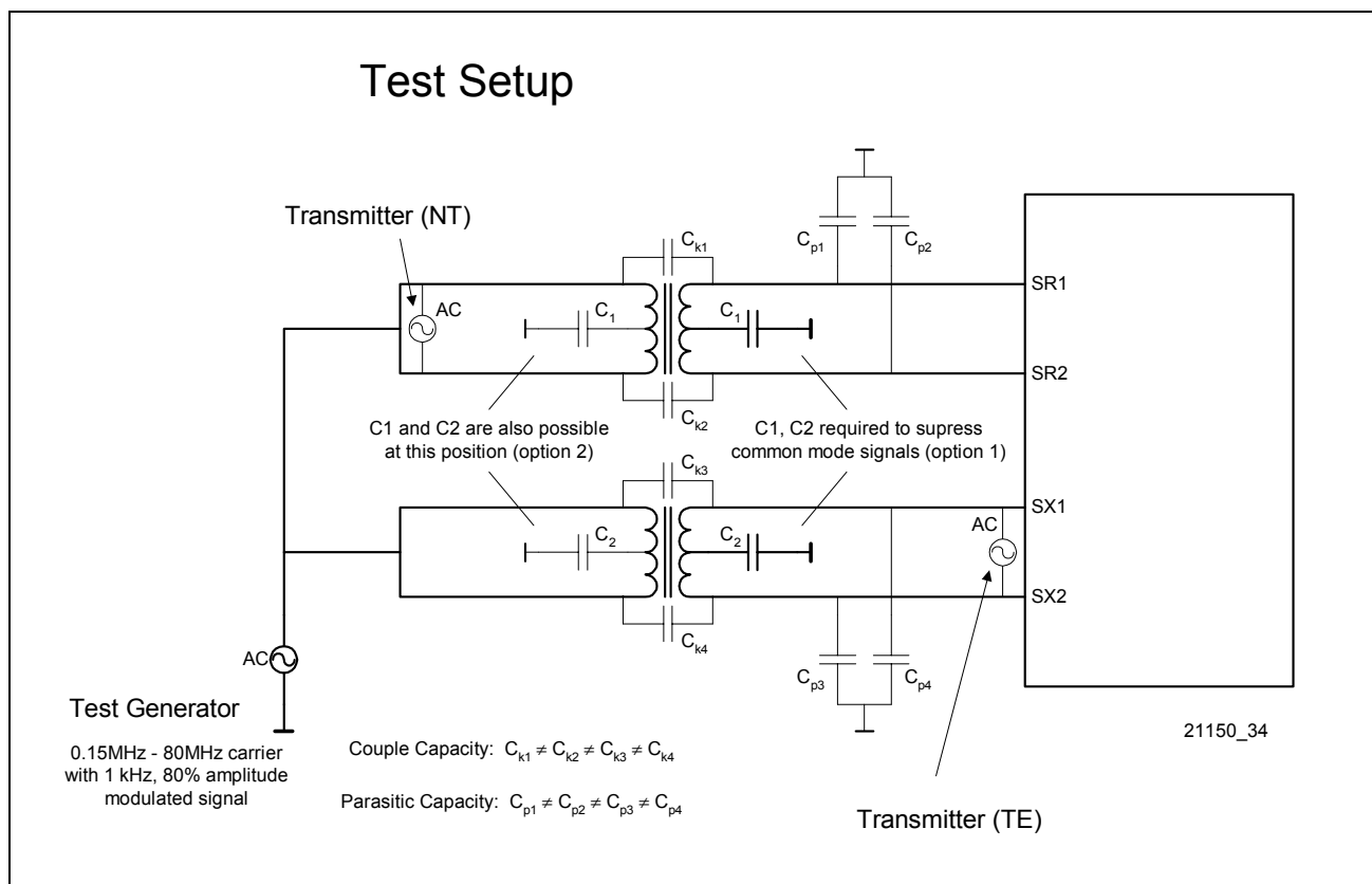
Figure 98 Transformer Circuitry
