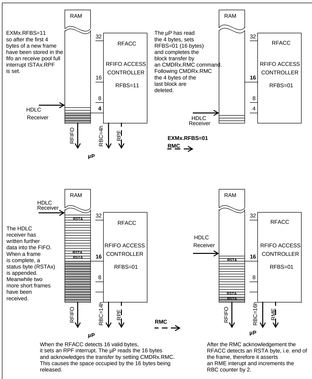
Figure 72 RFIFO Operation
