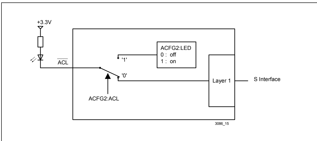
Figure 14 \overline{\text{ACL}} Configuration
