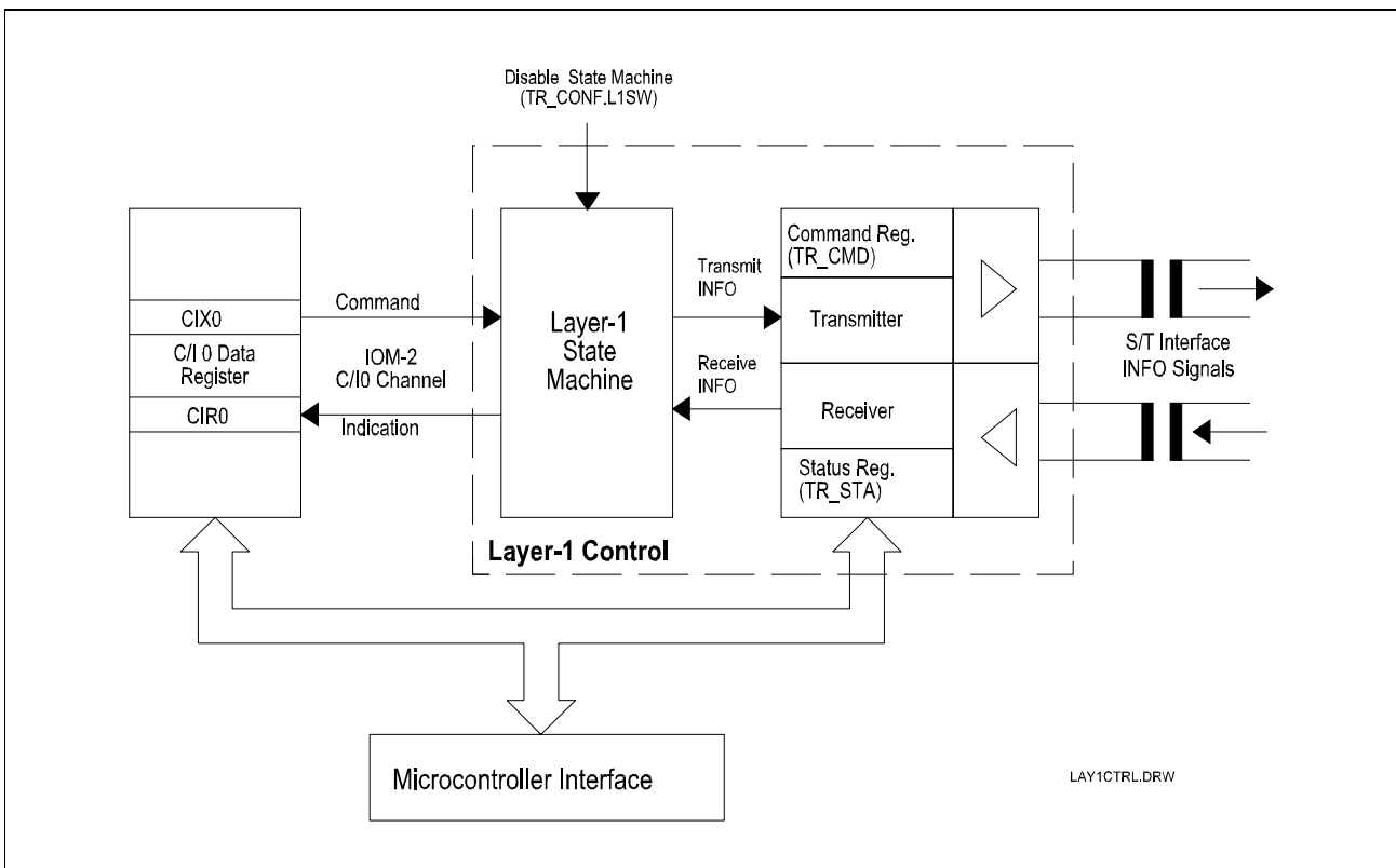
Figure 37 Layer-1 Control
