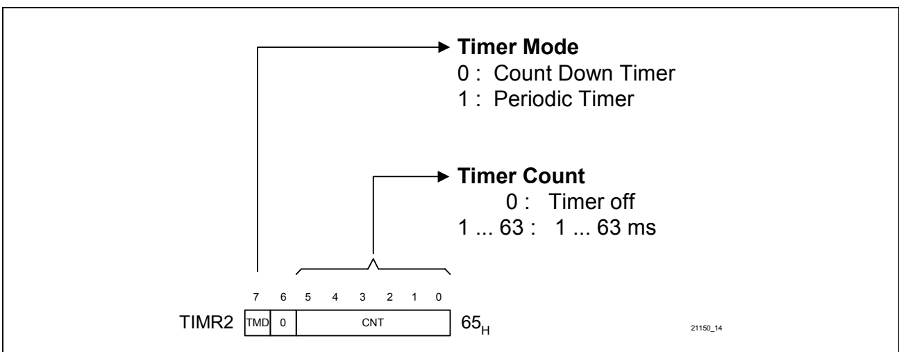
Figure 12 Timer 2 Register
