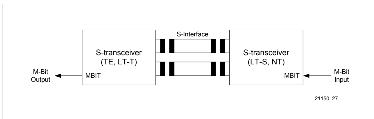
Figure 18 Multiframe Synchronization Using the M-Bit
