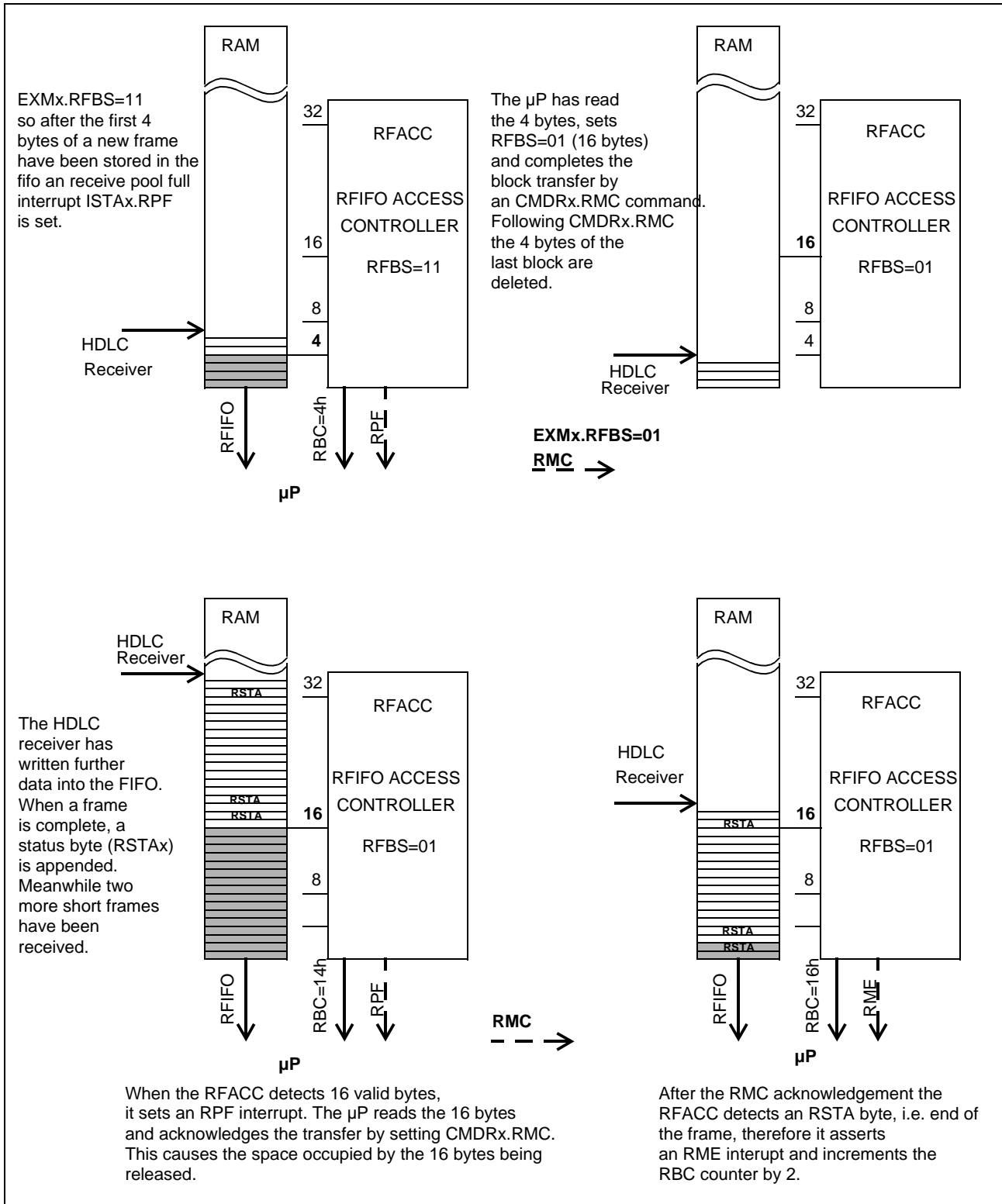
Figure 72 RFIFO Operation
