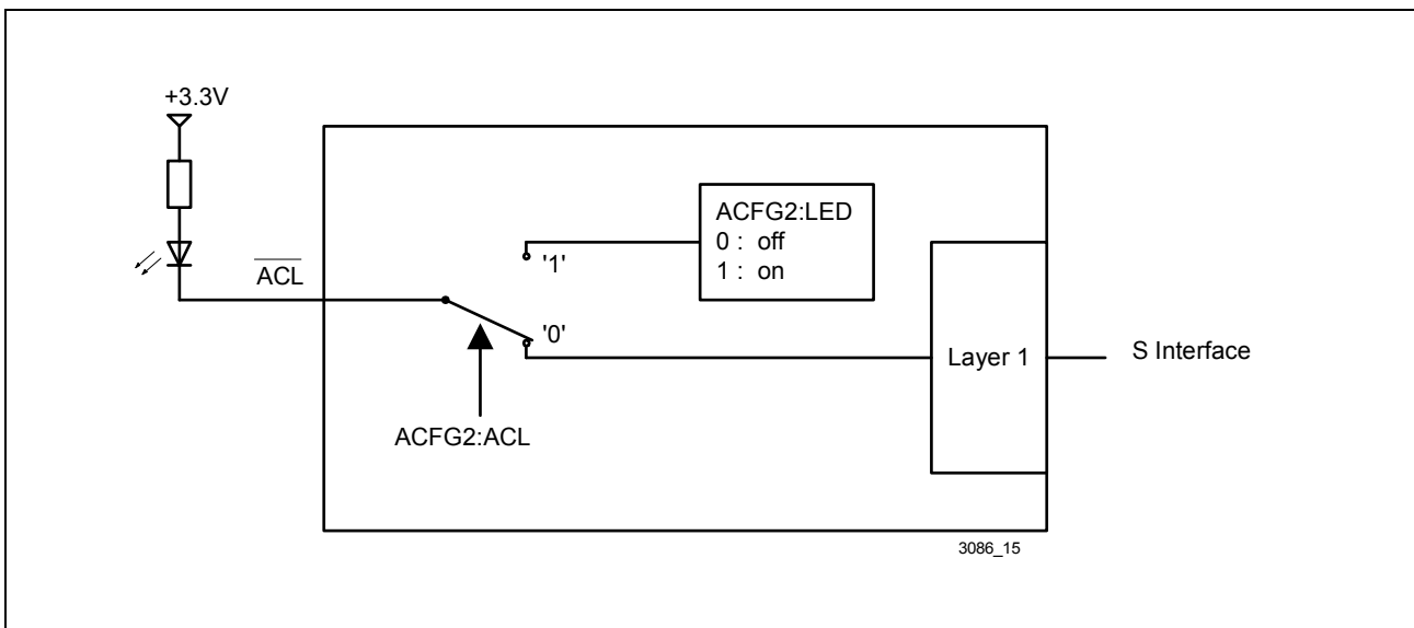
Figure 14 \overline{ACL} Configuration
