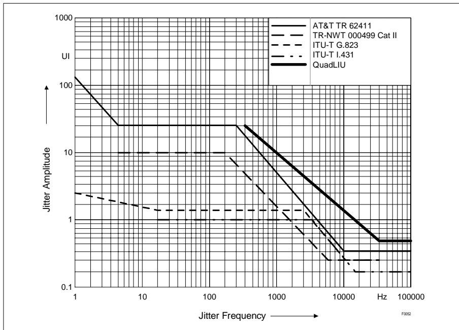
Figure 12 Jitter Tolerance
