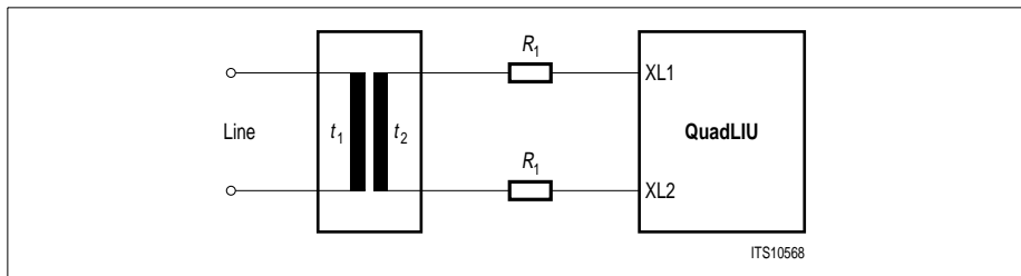
Figure 13 Transmitter Configuration
