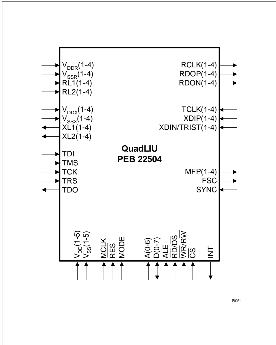
Figure 1 Logic Symbol
