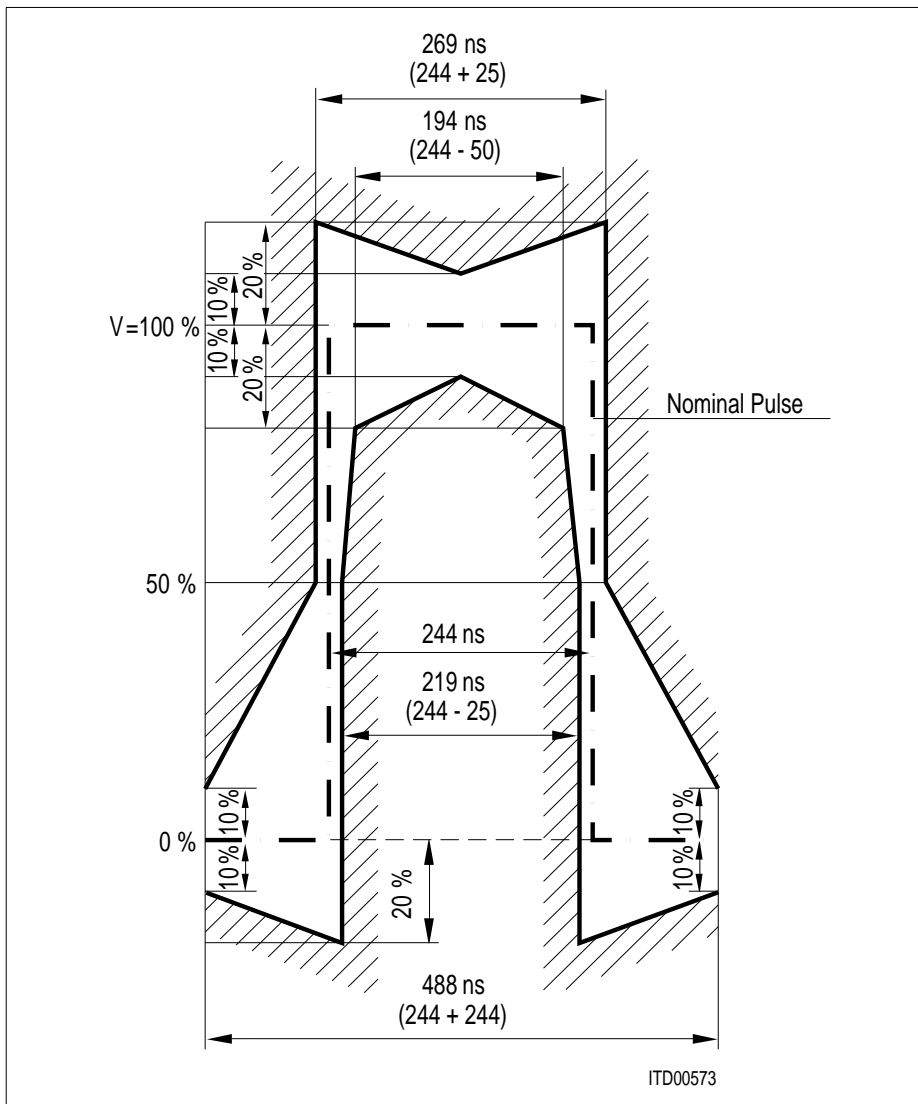
Figure 33 E1 Pulse Shape at Transmitter Output
