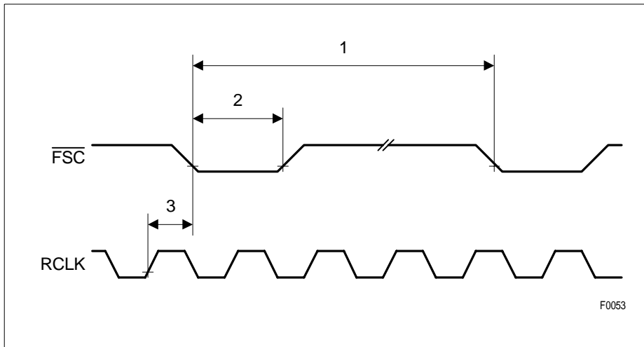
Figure 32 \overline{\text{FSC}} Timing
