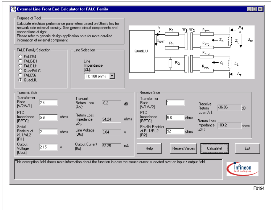
Figure 38 External Line Frontend Calculator
