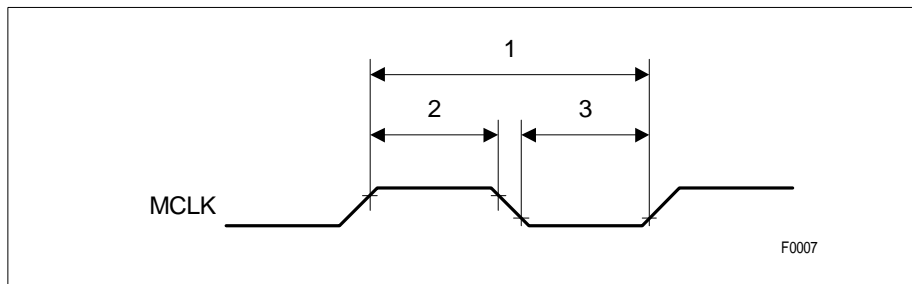
Figure 20 MCLK Timing
