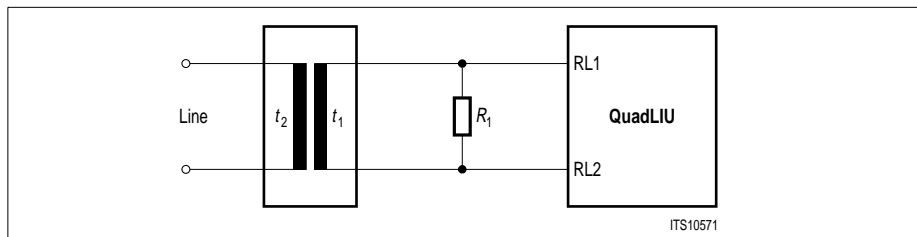
Figure 9 Receiver Configuration
