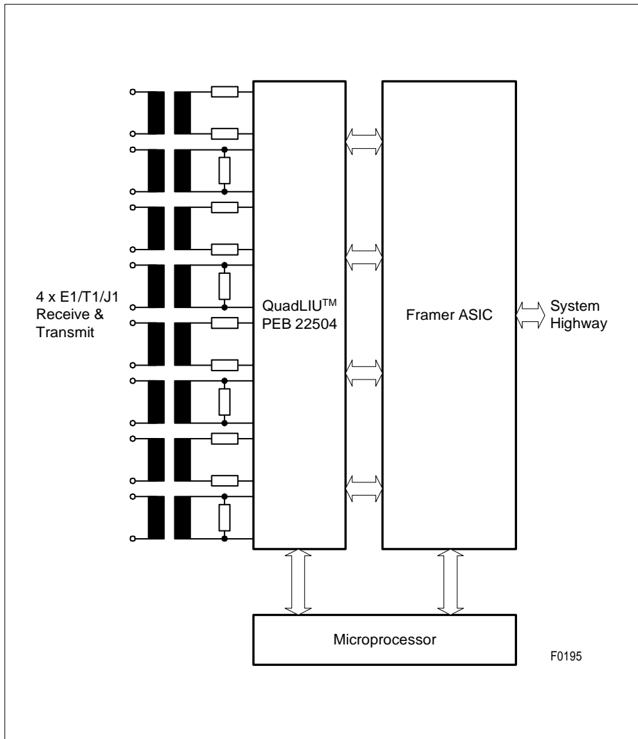
Figure 2 QuadLIU Application
