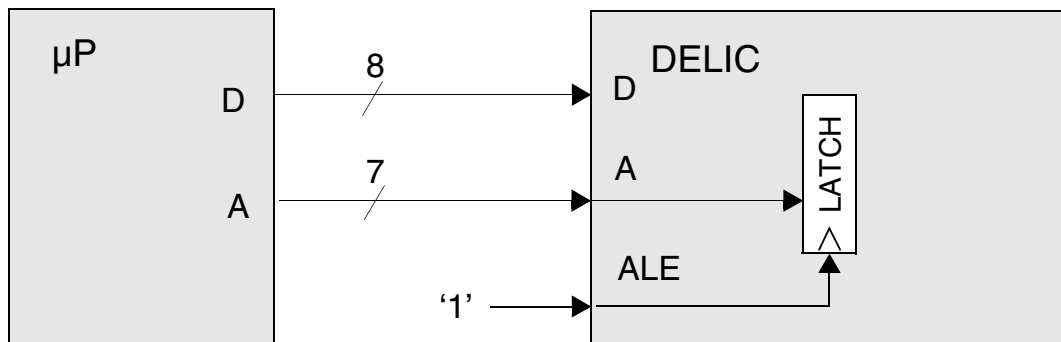
Figure 20 DELIC in Multiplexed and in De-Multiplexed Bus Mode
