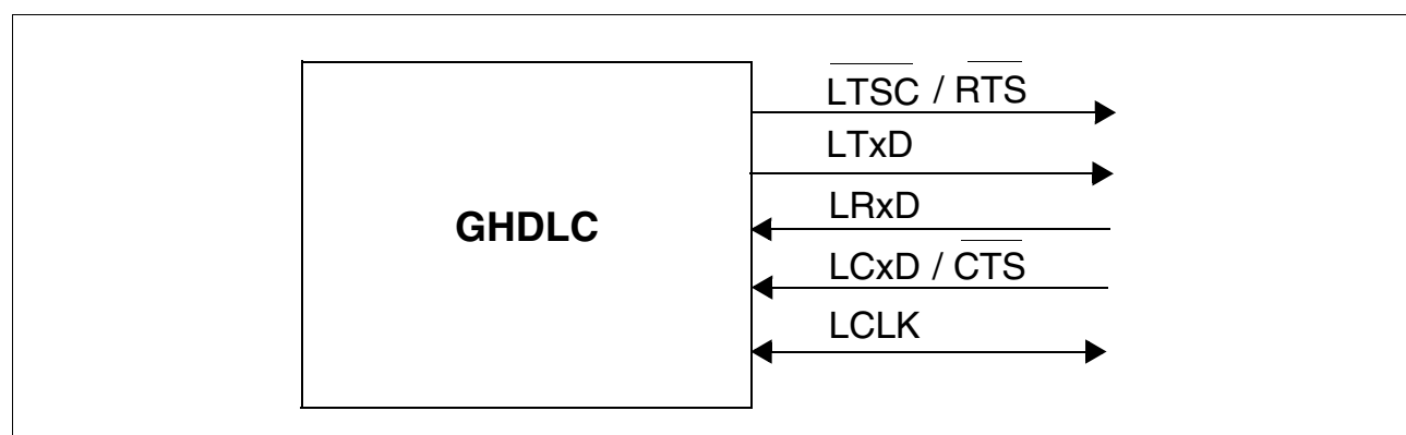
Figure 47 GHDLIC Interface Lines
