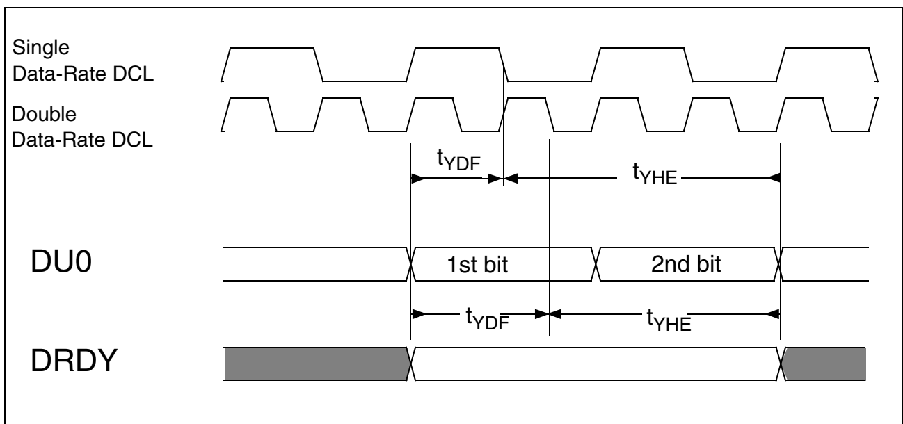
Figure 73 DRDY Timing
