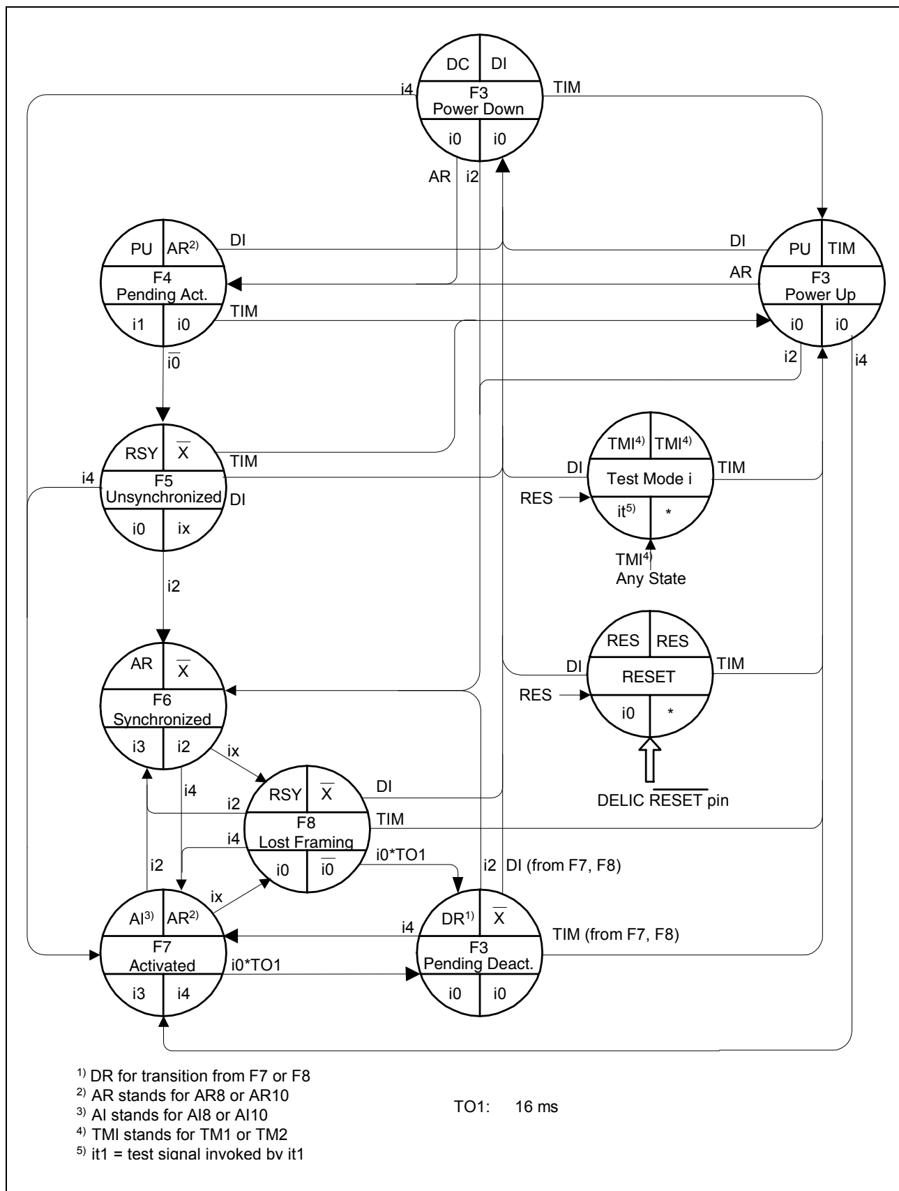
Figure 18 LT-T Mode State Diagram (Conditional and Unconditional States)
