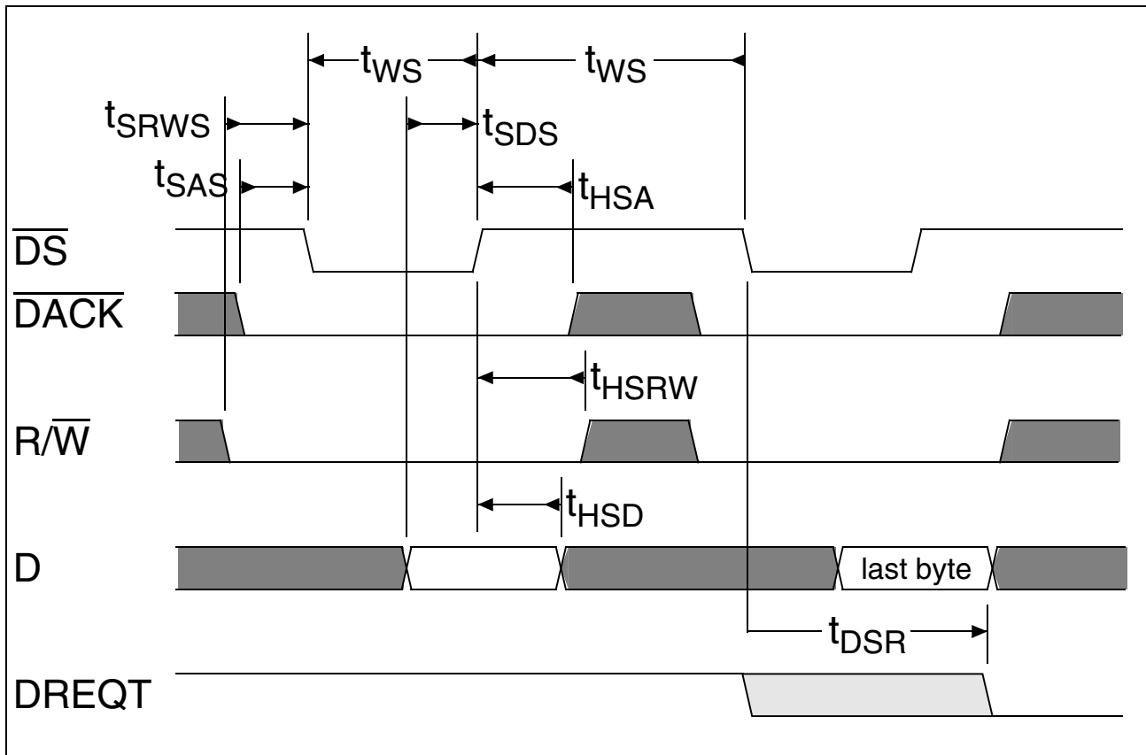
Figure 59 DMA Write-Transaction Timing in Motorola Mode
