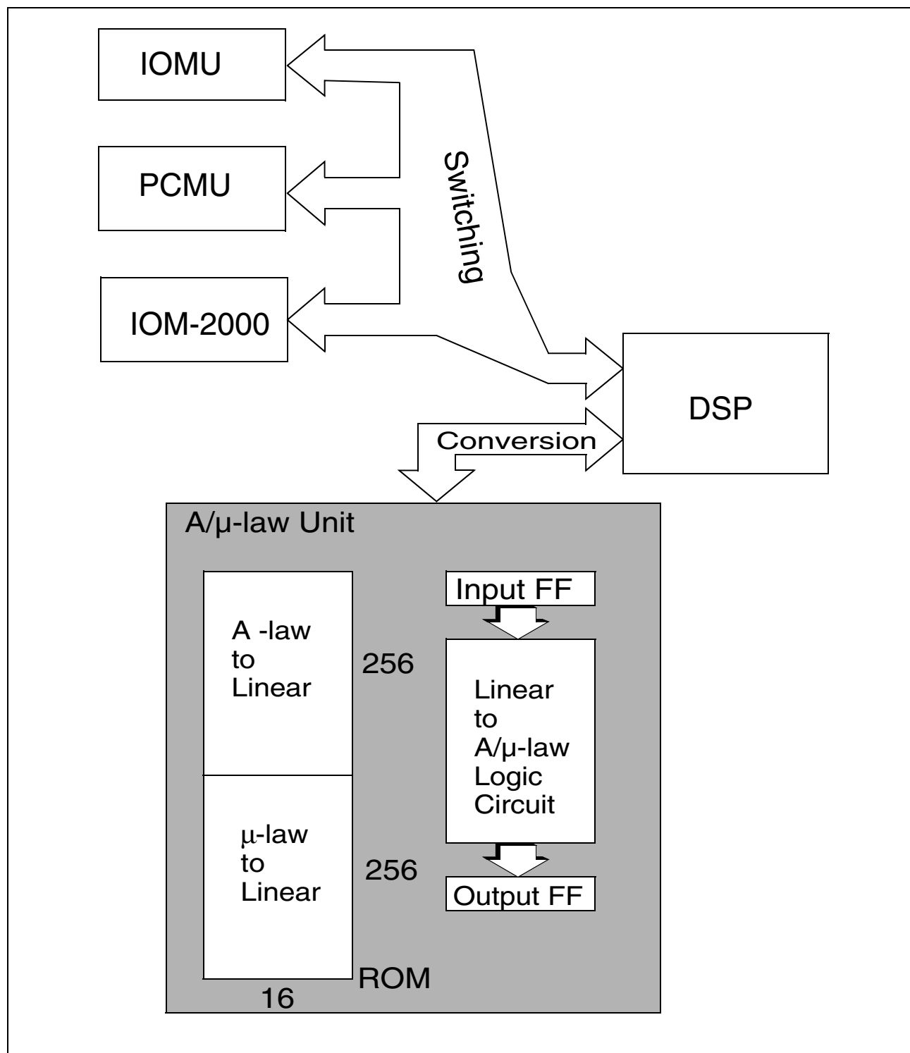
Figure 43 A-/μ-law Unit Integration
