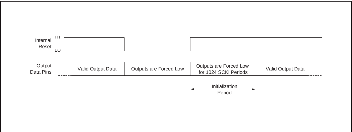
Figure 13. ADC Digital Output State for Reset Operations
