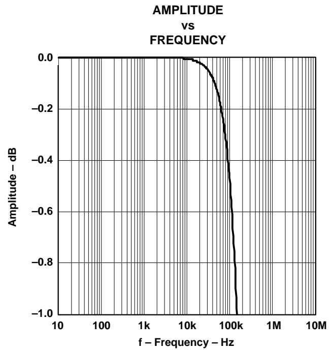
Figure 19. Analog Filter Pass-Band Performance (10 Hz–10 MHz)
