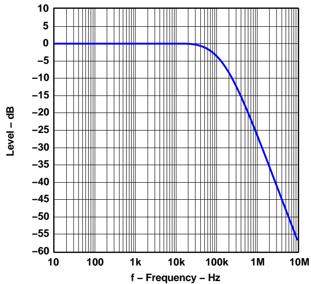
INTERNAL ANALOG FILTER FREQUENCY RESPONSE (10 Hz–10 MHz)
