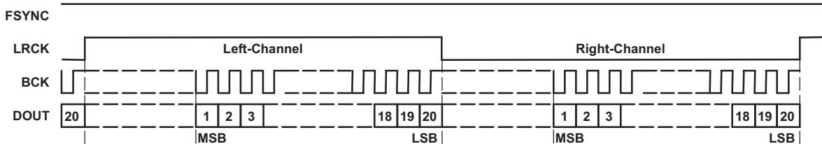
Figure 23. Audio Data Format (Slave Mode: FS SYNC , LRCK, and BCK Work as Inputs)
