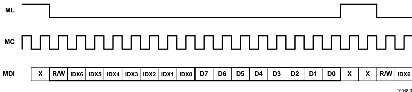
Figure 25. Write Operation Timing
