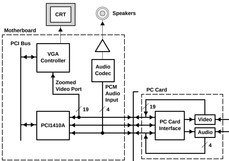
Figure 3-5. Zoomed-Video Implementation Using the PCI1410A Device
