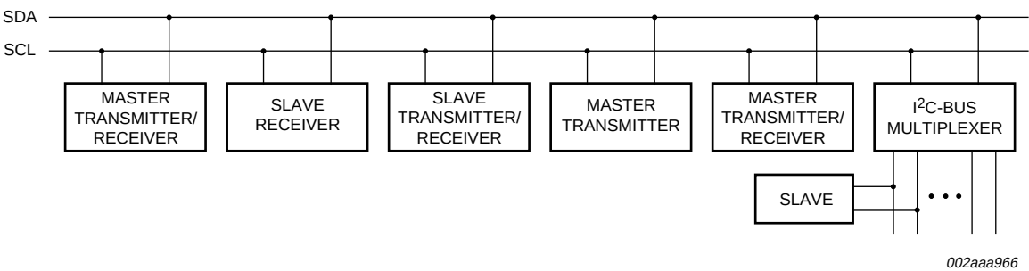
Fig 30. System configuration
