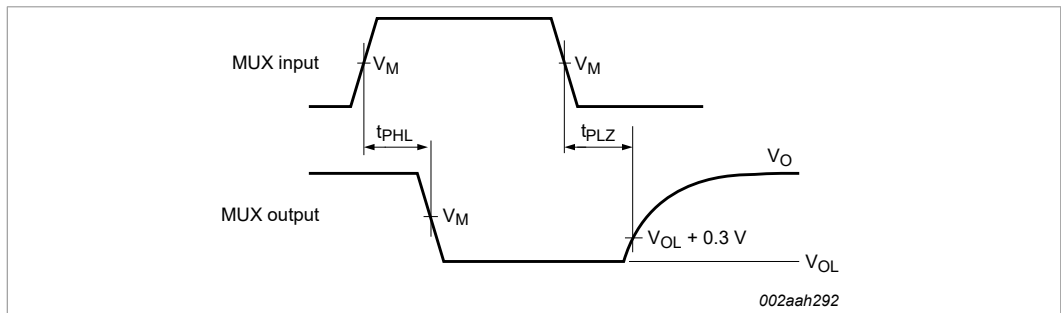
Figure 13. Open-drain output enable and disable times
