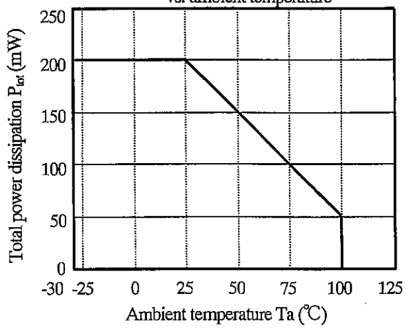
(Fig.6) Total power dissipation vs. ambient temperature
