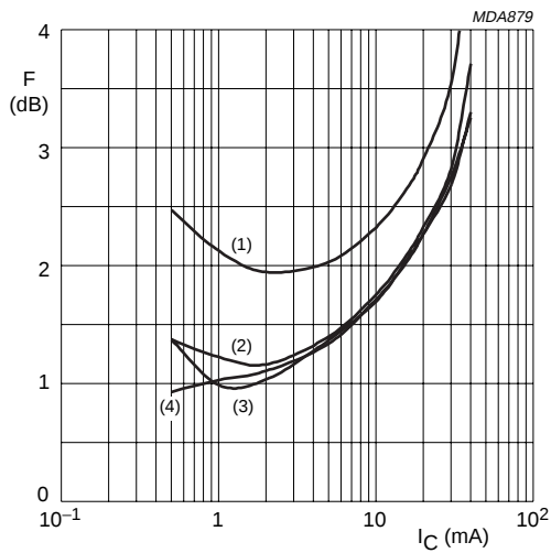
V_{CE} = 6\text{ V.} (1) f = 2000\text{ MHz.} (3) f = 500\text{ MHz.} (2) f = 1000\text{ MHz.} (4) f = 900\text{ MHz.}
