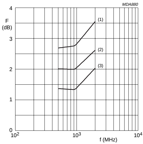
V_{CE} = 6\text{ V.} (2) I_C = 15\text{ mA.} (1) I_C = 30\text{ mA.} (3) I_C = 5\text{ mA.}
