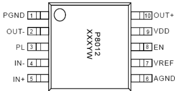
Top View eMSOP10
