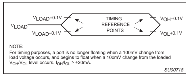
Figure 57. Float Waveform
