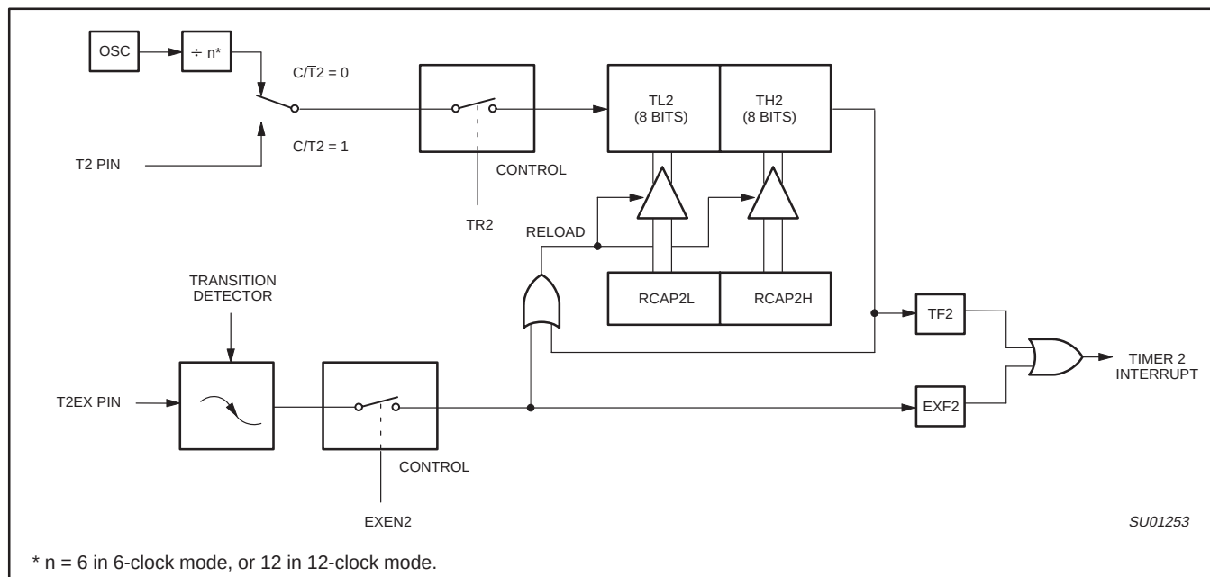
Figure 10. Timer 2 in Auto-Reload Mode (DCEN = 0)
