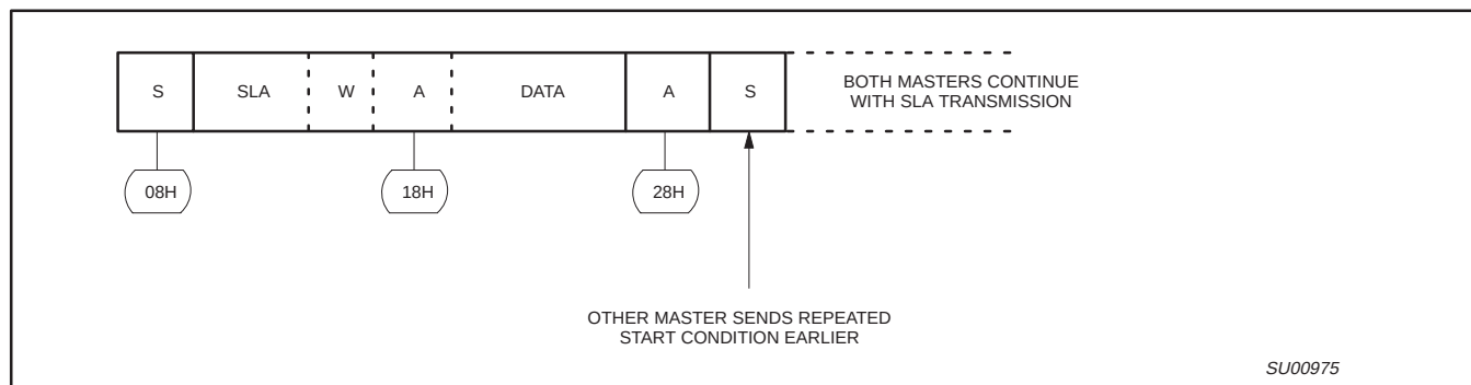
Figure 43. Simultaneous Repeated START Conditions from 2 Masters
