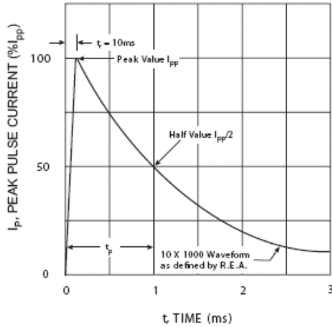
Fig. 1 Pulse Waveform
