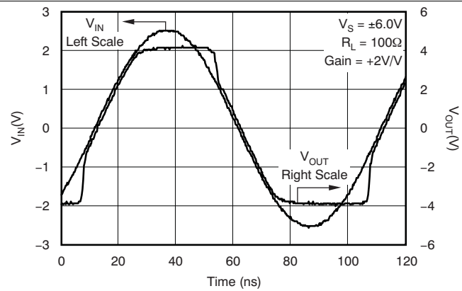
Figure 20. Overdrive Recovery (Gain = 2 V/V)
