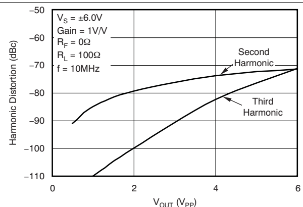
Figure 17. Harmonic Distortion vs Output Voltage
