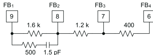
Figure 9-6. OPA836IRUN Gain-Setting Network
