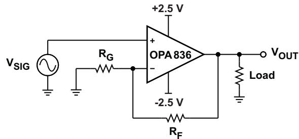
Figure 58. Split-Supply Operation
