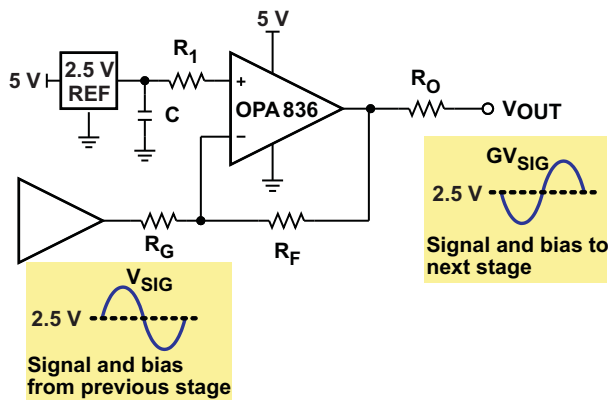
Figure 62. Inverting Single Supply With Reference
