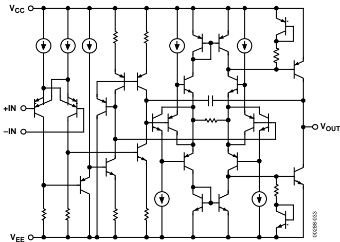
Figure 30. Simplified Schematic
