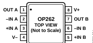
Figure 2. 8-Lead TSSOP (RU Suffix) and 8-Lead Narrow-Body SOIC (S Suffix)
