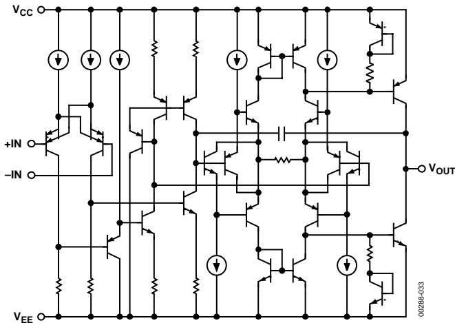
Figure 30. Simplified Schematic
