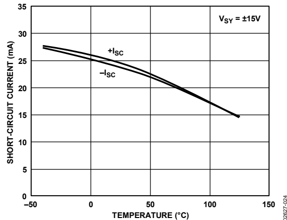
Figure 24. Short-Circuit Current vs. Temperature
