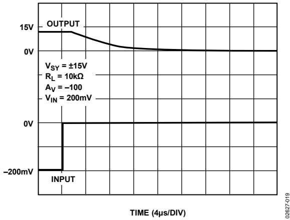
Figure 19. Negative Overtolerance Recovery
