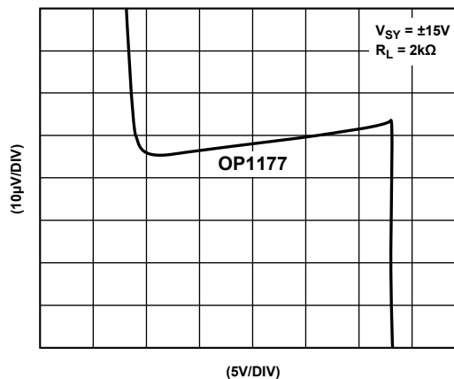
Figure 51. Gain Linearity
