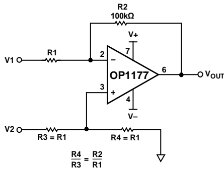
Figure 63. Difference Amplifier
