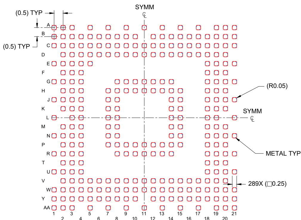
SOLDER PASTE EXAMPLE BASED ON 0.100 mm THICK STENCIL SCALE: 8X
