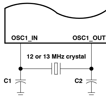
Figure 5-4. Internal System Oscillator External Crystal
