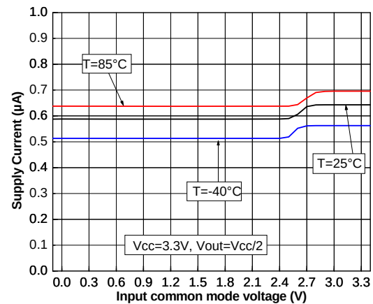
Figure 3. Supply current vs. input common mode voltage
