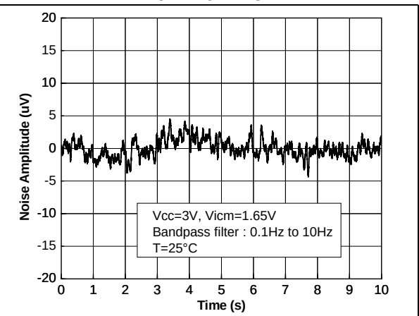
Figure 35. Noise amplitude on 0.1 to 10 Hz frequency range
