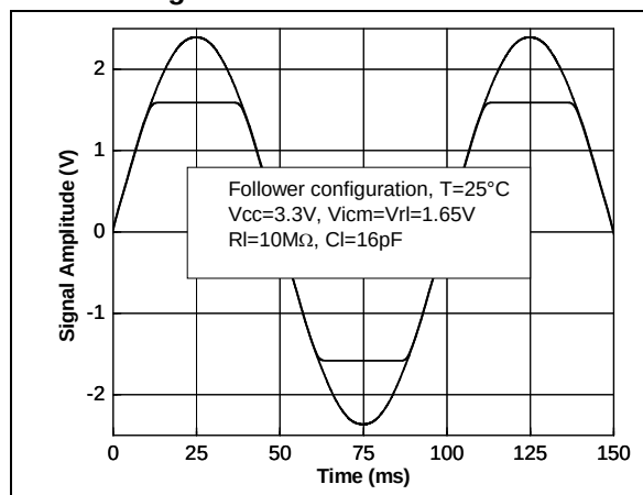
Figure 18. Phase reversal free
