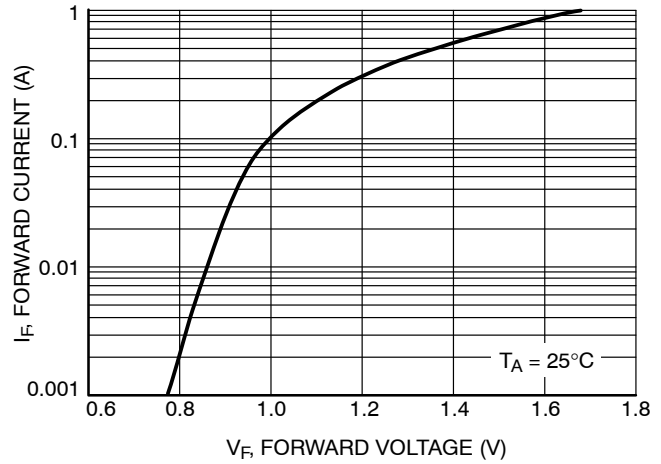
Figure 4. Forward Voltage
