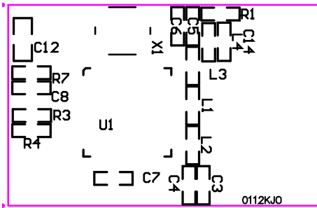
Top silk screen
