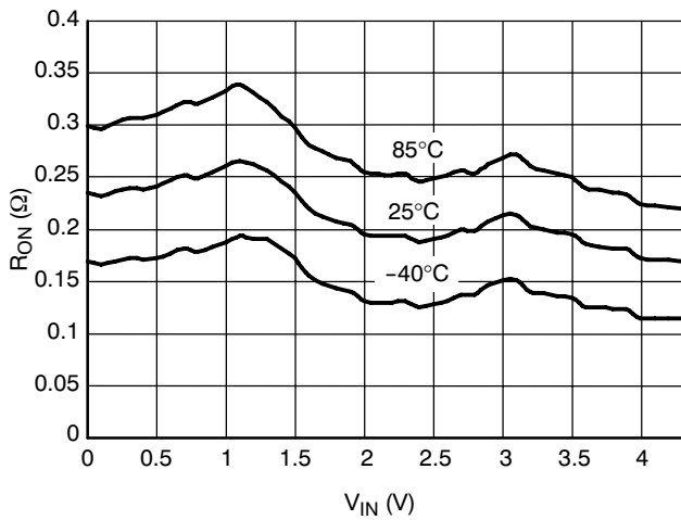
Figure 39. On-Resistance vs. Input Voltage @ V_{CC} = 4.2\text{ V}
