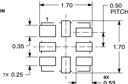
DIMENSIONS: MILLIMETERS
