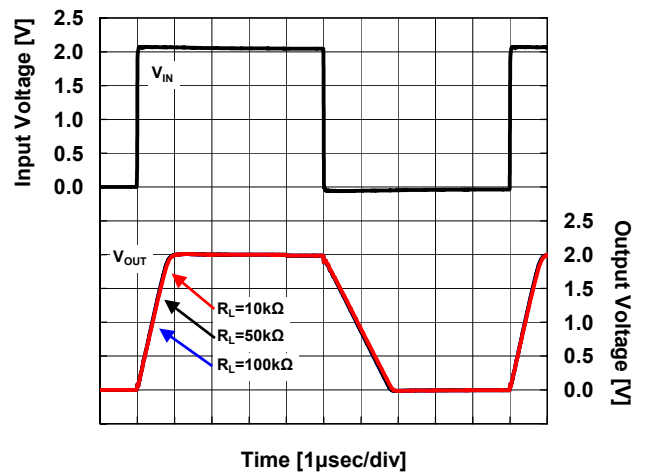
Pulse Response
