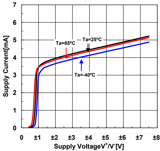
Supply Current vs. Supply Voltage (Temperature) G_V=0\text{dB}
