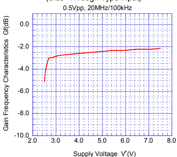
Gain Frequency Characteristics vs. Supply Voltage (Bias+Through Type Input)
