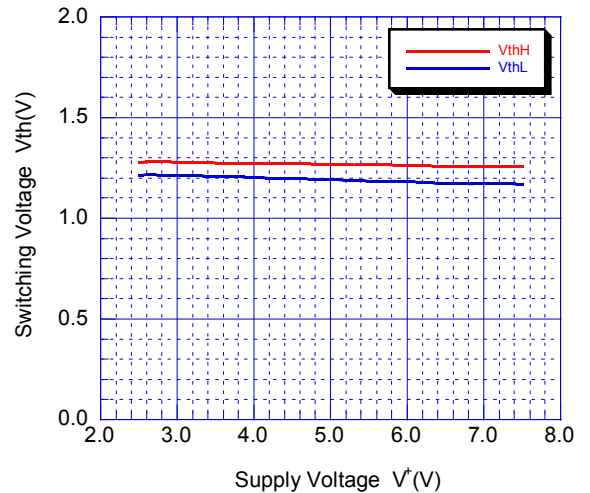
Switching Voltage vs. Supply Voltage
