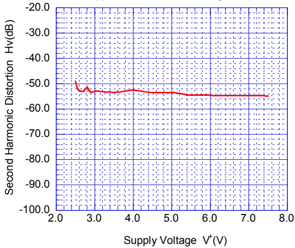
Second Harmonic Distortion vs. Supply Voltage 0.5Vpp, 3.58MHz sinewave signal input
